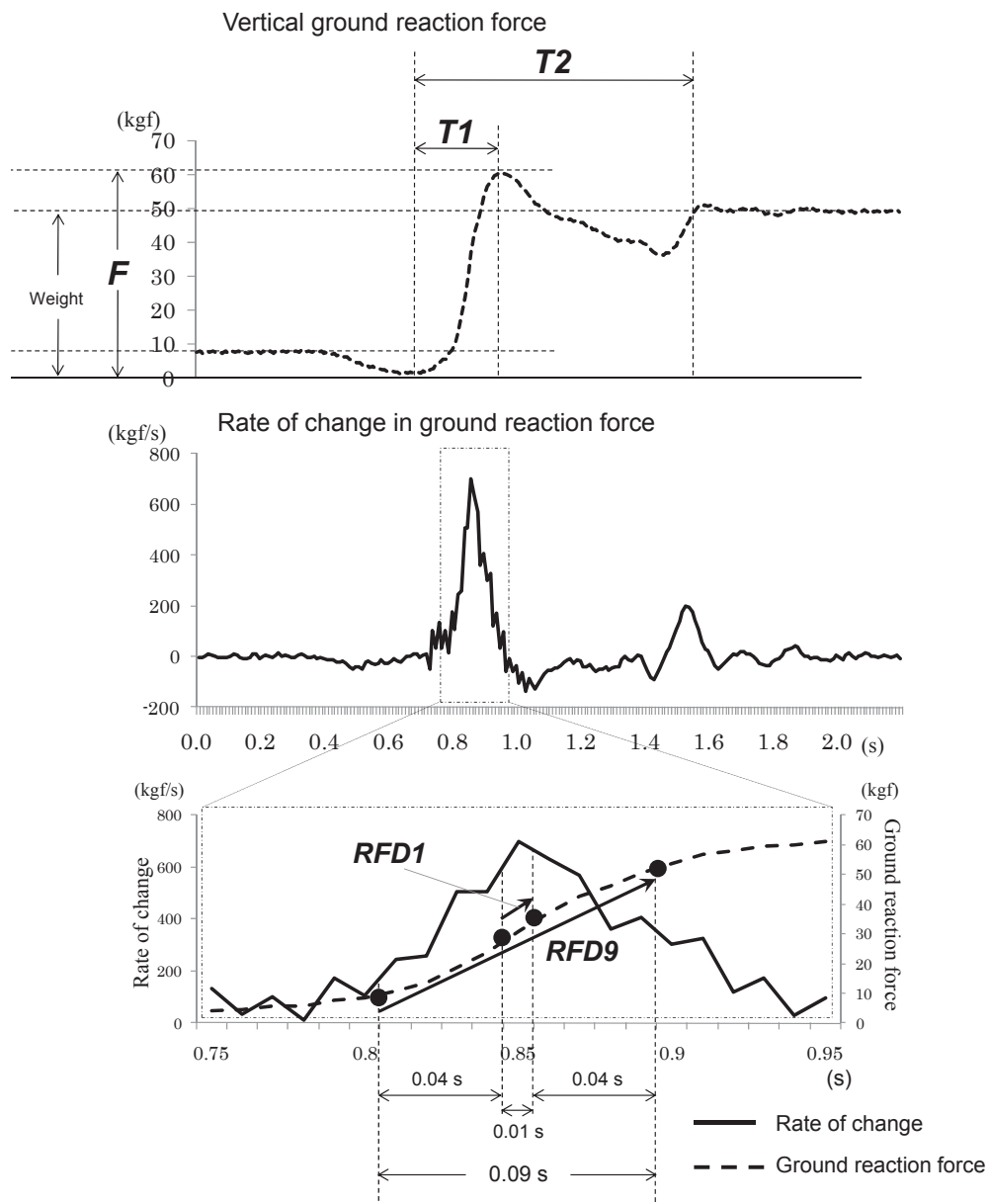
Figure 2. Ground reaction force parameters. F: peak reaction force; RFD1: the maximal rate of force development ( \Delta 10 ms); RFD9: the maximal rate of force development ( \Delta 90 ms); T1: time span of the developing force; T2: chair-rise time.
